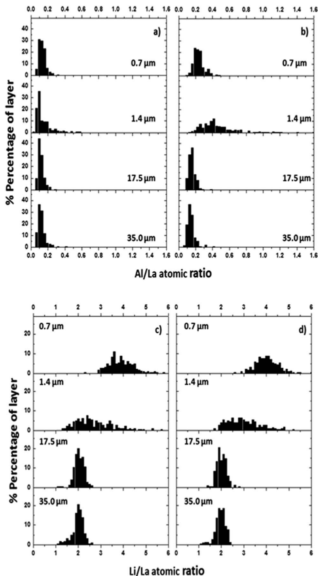
Fig. 5 Distributions of atomic ratios across selected layers depths from the sample surface (0.7, 1.4, 17.5, 35.0 \mu\text{m} ). The atomic ratio of Al/La is shown in (a) for LLZO_0h and (b) for LLZO_6h. The Li/La atomic ratio is shown in (c) and (d) for LLZO_0h and LLZO_6h respectively.
