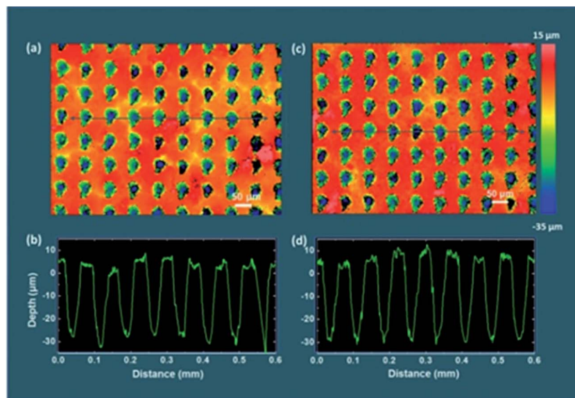
Fig. 1 White light interferometry surface maps of the laser-sampled areas for (a) LLZO_0h and (c) LLZO_6h. (b and d) Corresponding line profiles of the craters across the horizontal blue lines shown in (a) and (c).
