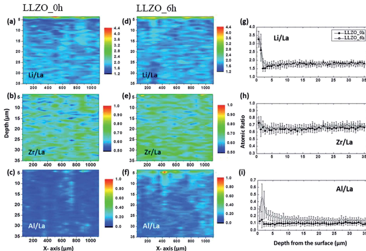
Fig. 6 Atomic ratio (Li/La, Zr/La, Al/La) maps as a function of depth across a section of the two LLZO samples (a–f), and mean atomic ratio as a function of depth (g–i). The error bars represent the standard deviation in the atomic ratios across each lateral plane.
