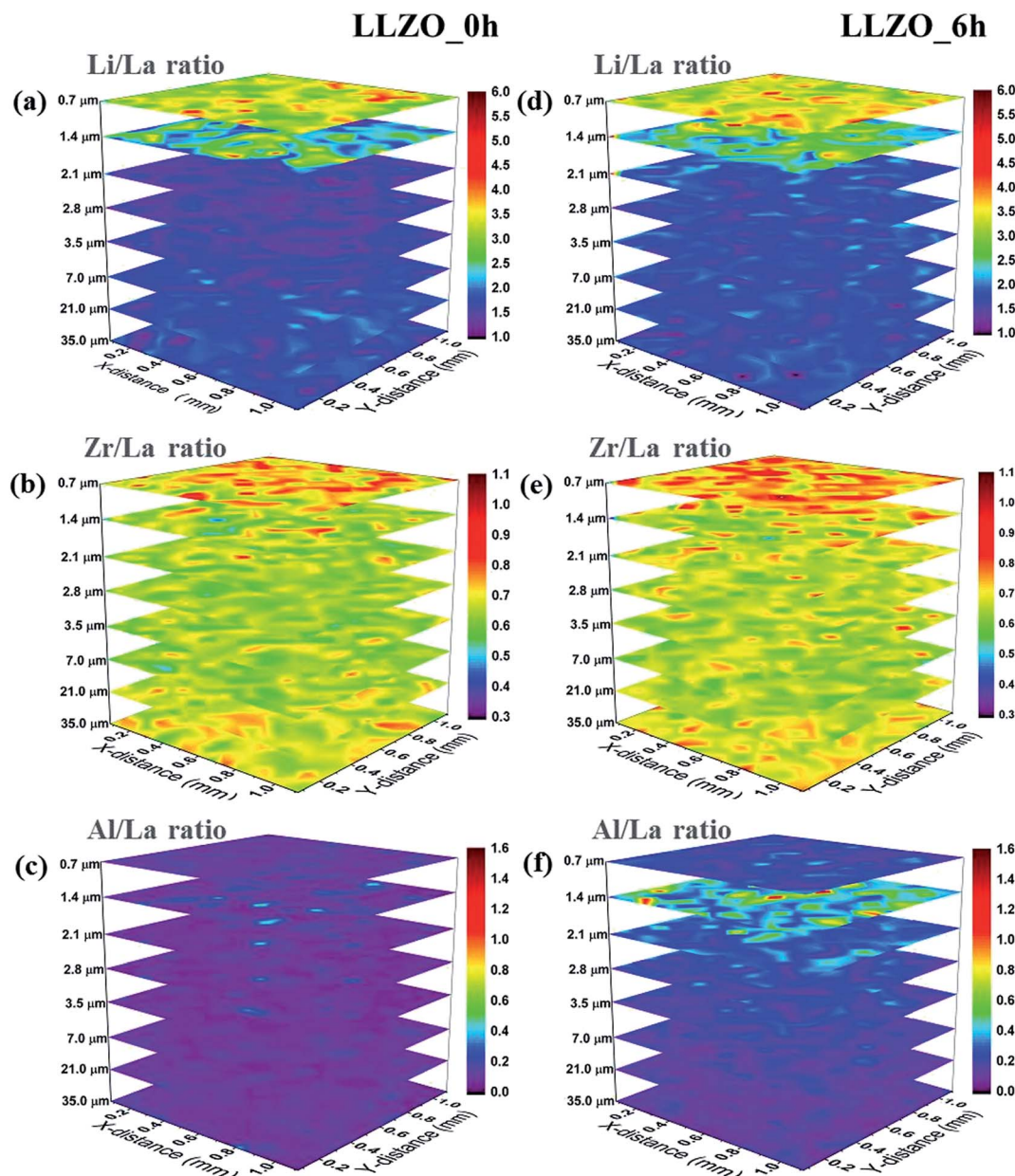
Fig. 4 Atomic ratios for major and minor elements in two LLZO pellets prepared under different conditions, for the first 35 \mu\text{m} from the surface. (a) Li/La, (b) Zr/La and (c) Al/La ratios for LLZO_0h. (d) Li/La, (e) Zr/La and (f) Al/La ratios for LLZO_6h. The depth/pulse is 700 nm (total sampled area/layer: 1.11 mm \times 1.11 mm). Al-rich areas are found at the surface (0.7 to 2.1 \mu\text{m} in depth) of LLZO_6h (f).
