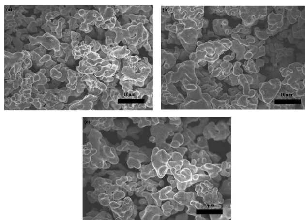
Fig. 2 SEM images of (a) fresh powder (b) powder annealed for 6 h, (c) and powder annealed for 12 h.
