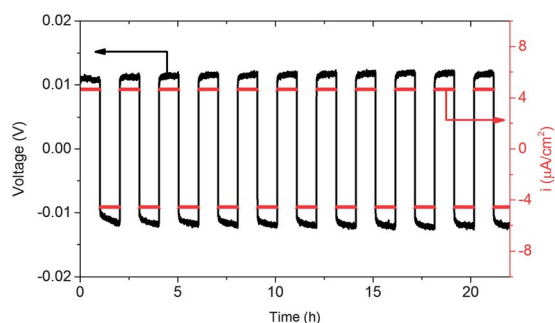
Fig. 13 Galvanostatic cycling of a symmetrical cell with lithium electrodes and LLZO sintered in fresh powder at current density of 4.6 \mu\text{A cm}^{-2} . The LLZO pellet used for this experiment was approximately 1.5 mm thick and 8.0 mm in diameter and was processed in fresh powder without polishing.
