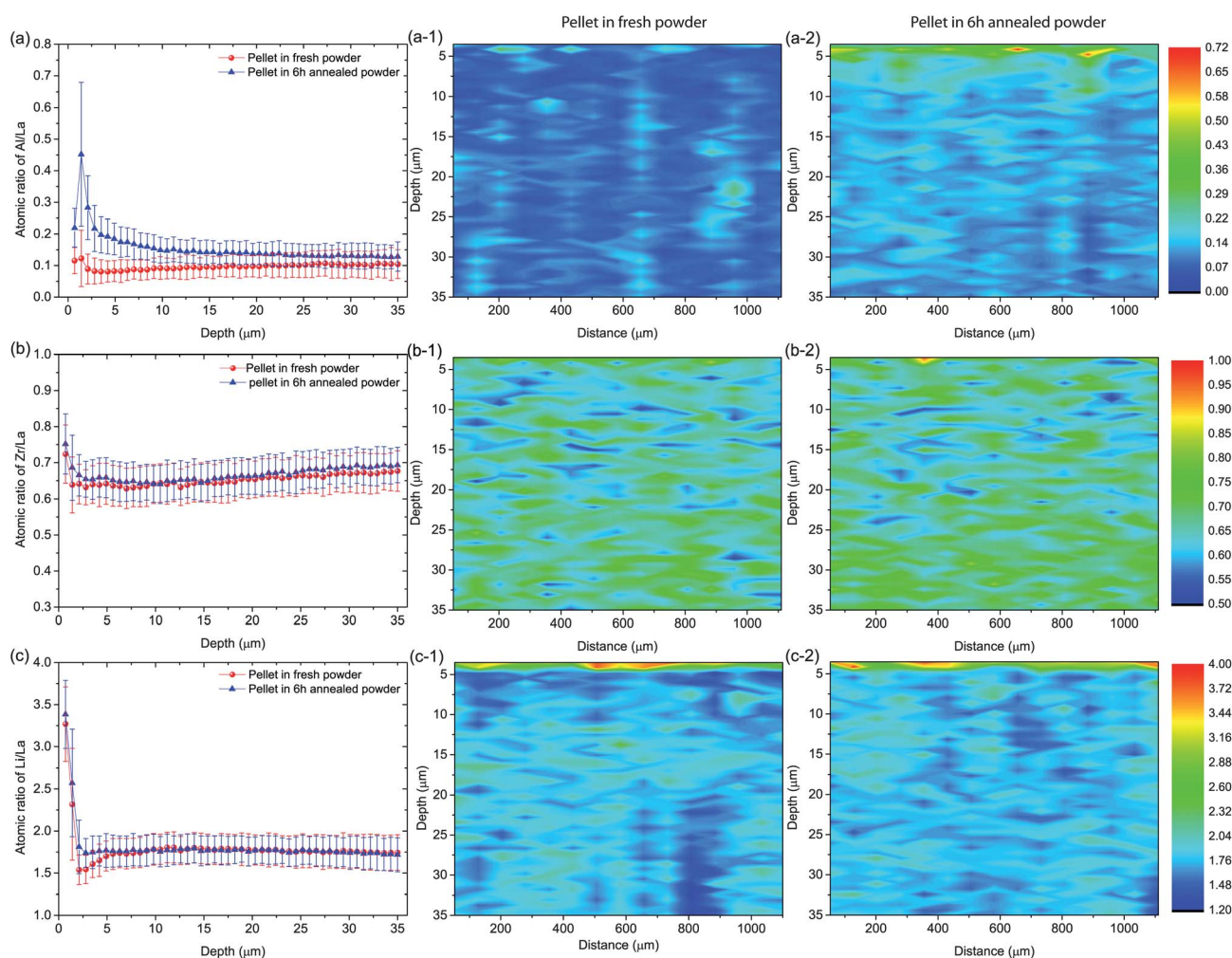
Fig. 10 LIBS depth profiles (a–c) and cross-section imaging (a-1–c-2) of Al/La (a, a-1, and a-2), Zr/La (b, b-1, and b-2) and Li/La atomic ratios (c, c-1, and c-2) of pellets made in fresh powder and the powder annealed for 6 h.
