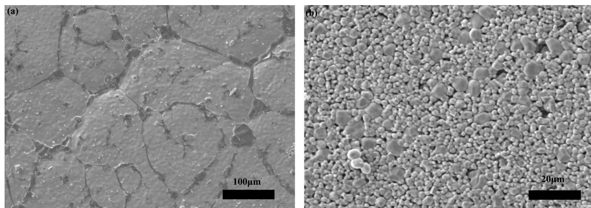
Fig. 7 SEM images of the pellets sintered in (a) 6 h annealed (b) 12 h annealed LLZO powder covers.
