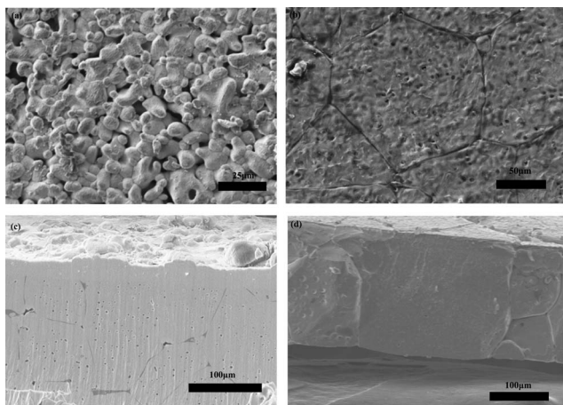
Fig. 6 (a) Pellet made using unmilled fresh powder, (b) pellet made from the attrition milled powder, (c) Ar-ion milled cross section of a pellet made from the attrition milled powder, and (d). Cross-section produced by fracturing a single-grain thick film made from attrition milled powder.
