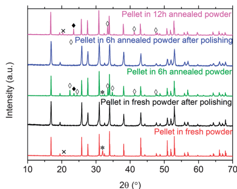
Fig. 9 XRD patterns of a pellet sintered in fresh powder (bottom), a pellet sintered in fresh powder after polishing (second from bottom), a pellet sintered in 6 h annealed powder (third from bottom), a pellet sintered in 6 h annealed powder after polishing (second from top) and, a pellet sintered in 12 h annealed powder (top). ◇ \text{LiAlO}_2 (PDF# 018-0714); ◆ \text{LaAlO}_3 (PDF# 085-1071); * \text{La}_2\text{Li}_{0.5}\text{Al}_{0.5}\text{O}_4 (PDF# 040-1167); × \text{Li}_2\text{ZrO}_3 (PDF# 016-0263).
