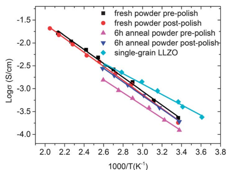
Fig. 11 Total ionic conductivities of pellets prepared in fresh powders or those annealed for 6 h, before and after polishing. Also shown is data for the single grain LLZO film similar to that shown in Fig. 6d.
