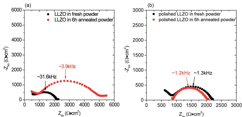
Fig. 12 Nyquist plots of symmetrical cells containing thick pellets sandwiched between lithium electrodes. The plot on the left shows data for pellets processed in fresh or annealed powders before polishing and the one on the right shows the results after the pellets were polished.
