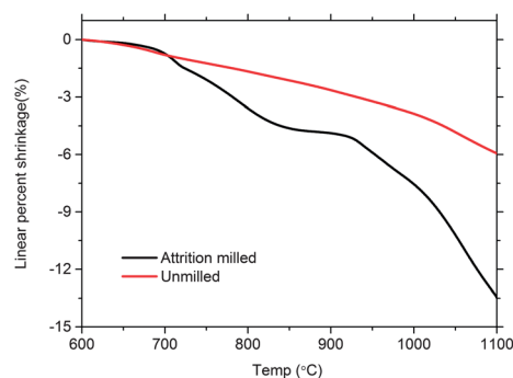
Fig. 5 Dilatometry sintering profiles from 600 °C to 1100 °C of pellets made from attrition milled and unmilled powders.
