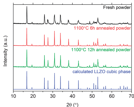
Fig. 3 XRD patterns of fresh powder (top), powder annealed in \text{Al}_2\text{O}_3 crucible at 1100 °C for 6 h (second from top), powder annealed in \text{Al}_2\text{O}_3 crucible at 1100 °C for 12 h (second from bottom) and simulated cubic LLZO pattern simulated based on ref. 6.
