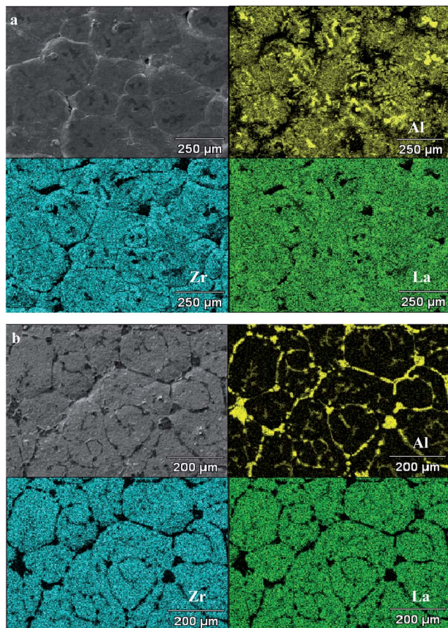
Fig. 8 EDS spectral imaging of (a) a pellet sintered in fresh powder cover (b) a pellet sintered in 6 h annealed powder cover.
