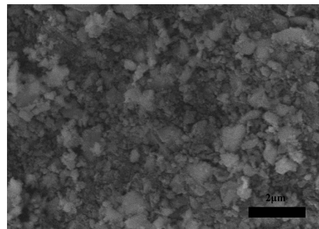
Fig. 4 SEM images of attrition milled particles.
