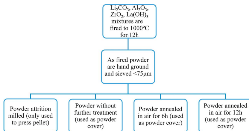
Fig. 1 Schematic of the LLZO powder processing.
